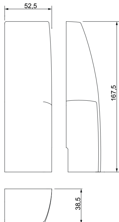
Deckel Art. 09775
