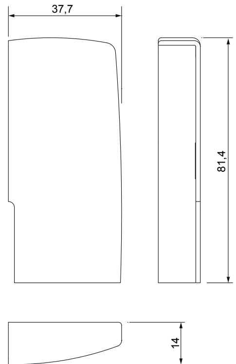
Deckel Art. 09774
