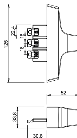
Overall dimensions art. 01079
