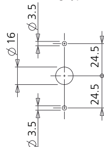
Machining type 3
