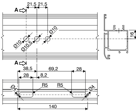
Type C: machining
