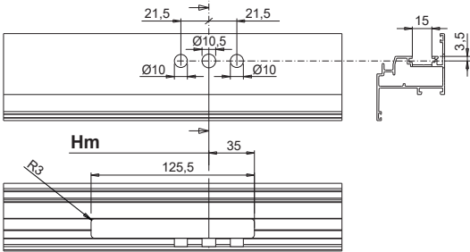
Type D: machining
