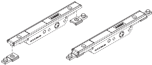
Assembly with movement 0102001
