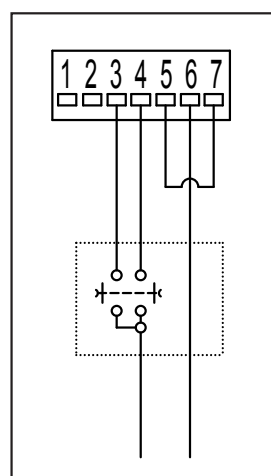
Wiring diagram
