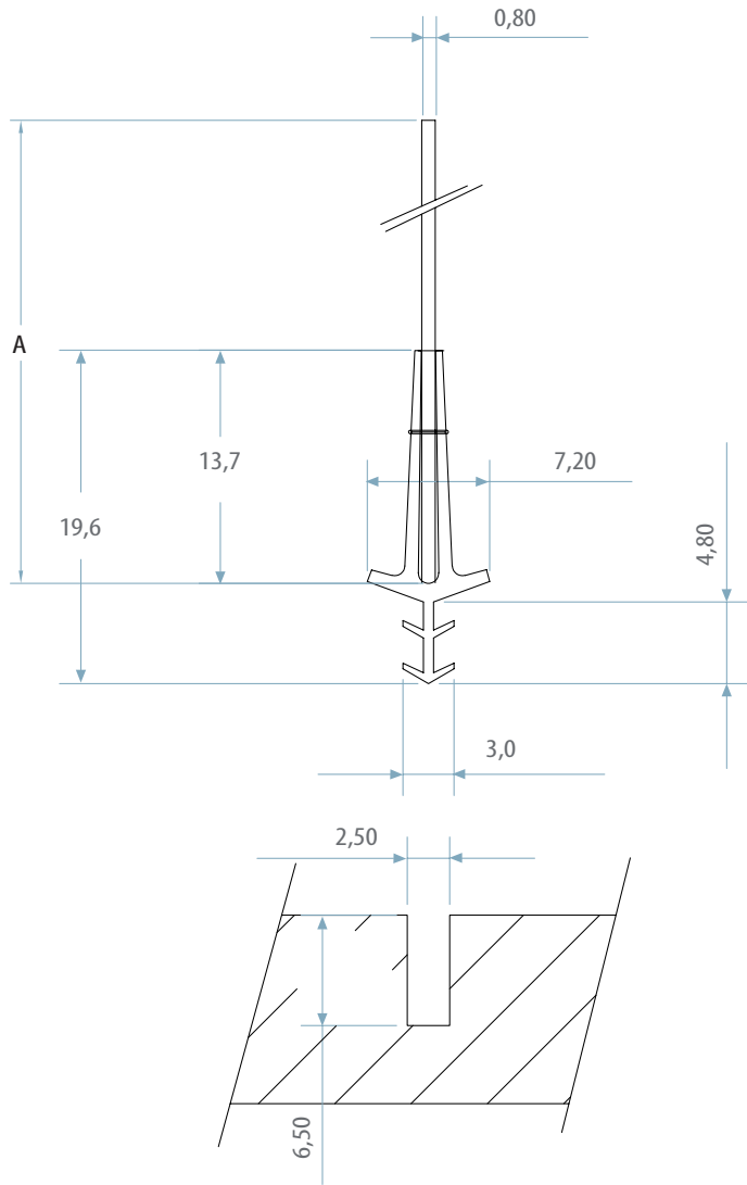
Recommended sawcut dimensions
